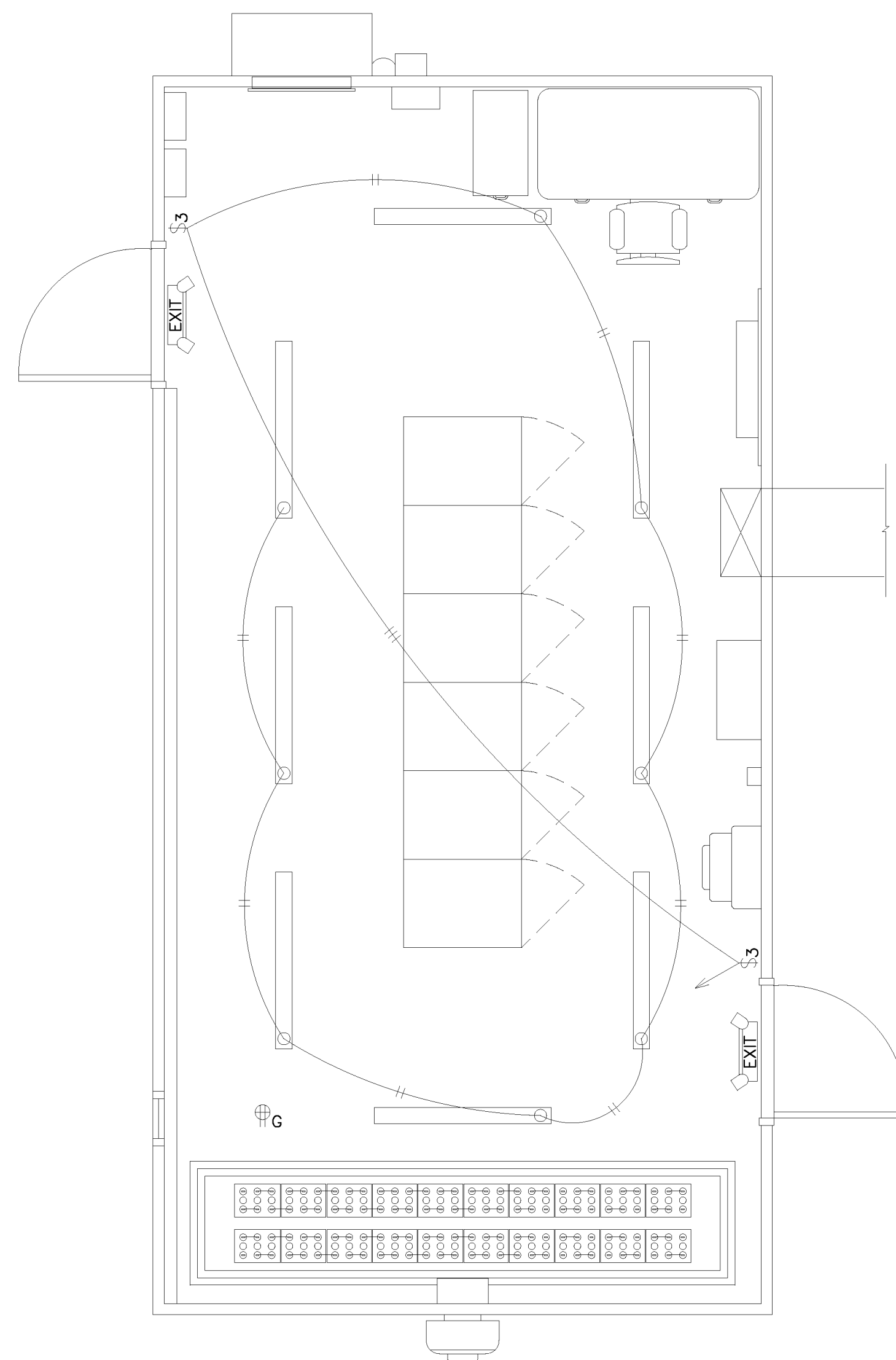
CONTROL ROOM LIGHTING PLAN
