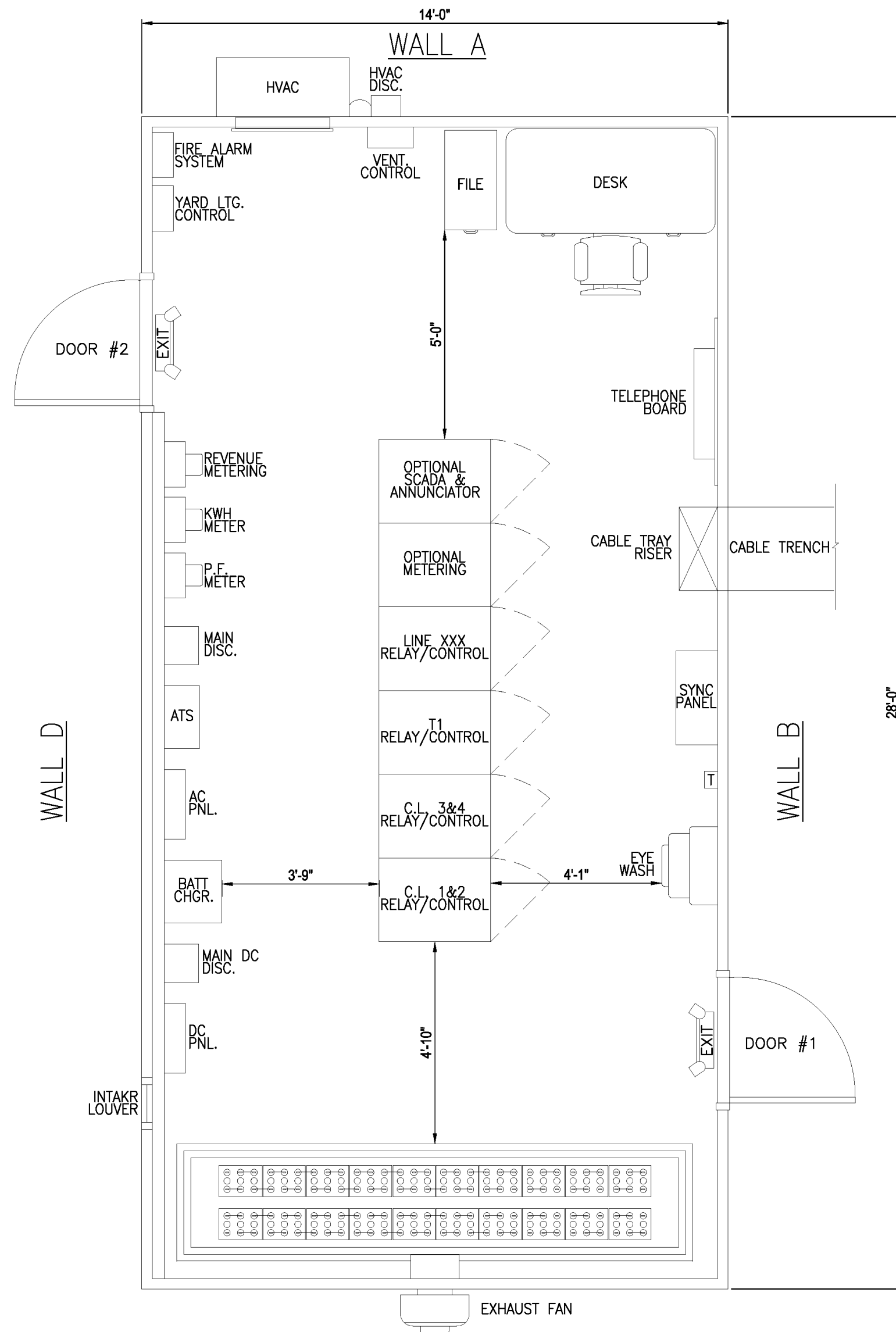
WALL C CONTROL ROOM FLOOR PLAN
